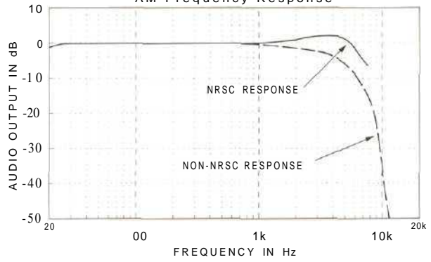
AM Frequency Response
